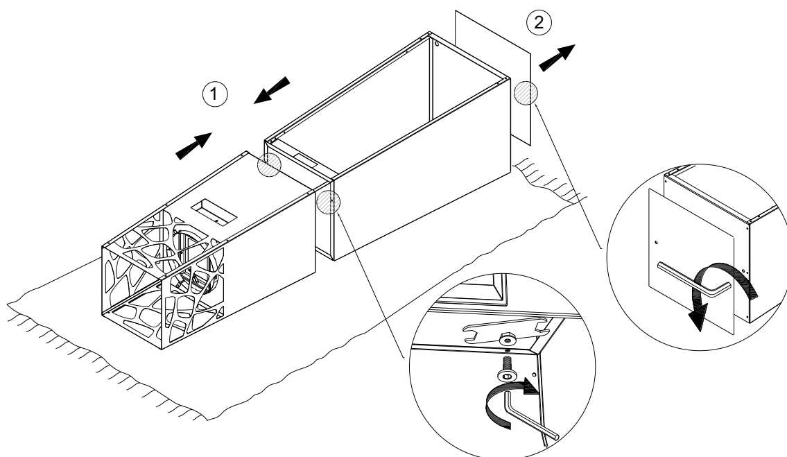
Fig. 6 – Connecting fireplace parts together and unscrewing the protective cover
