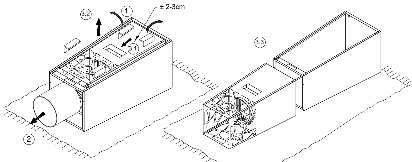
Fig. 5 – Unboxing the fireplace
