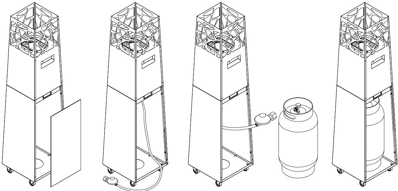
Fig 9– Gas cylinder installation
