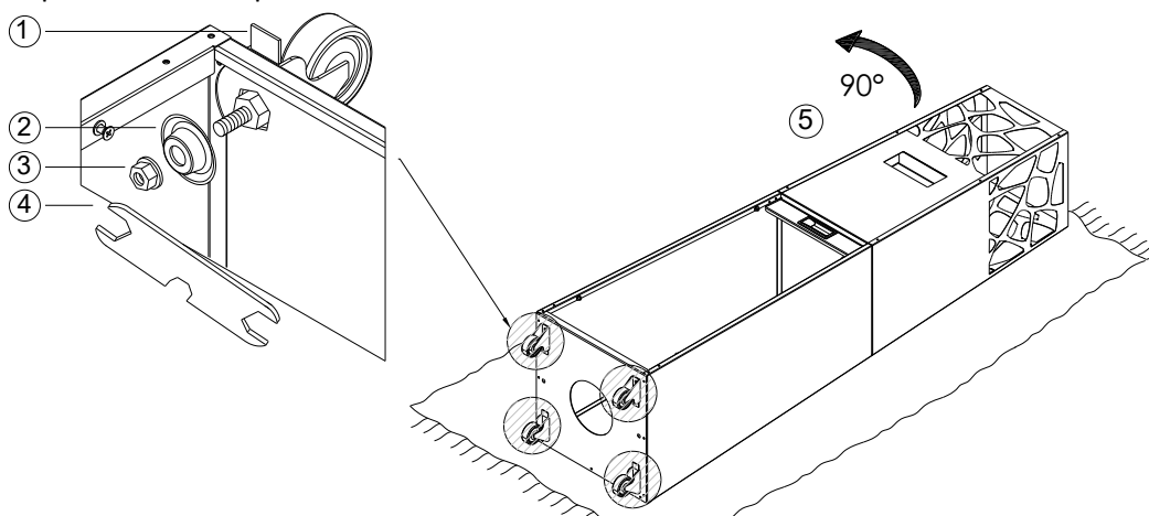
Fig. 7 – Installing the wheels
