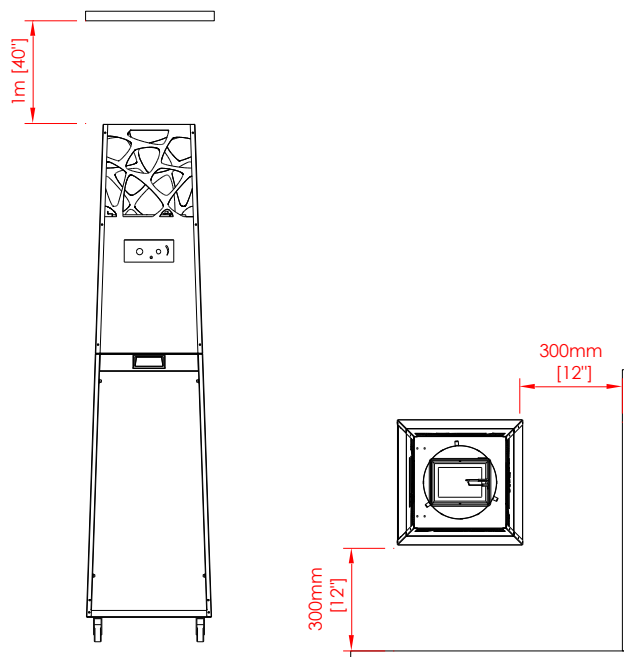
Fig 2 – Distances minimales
