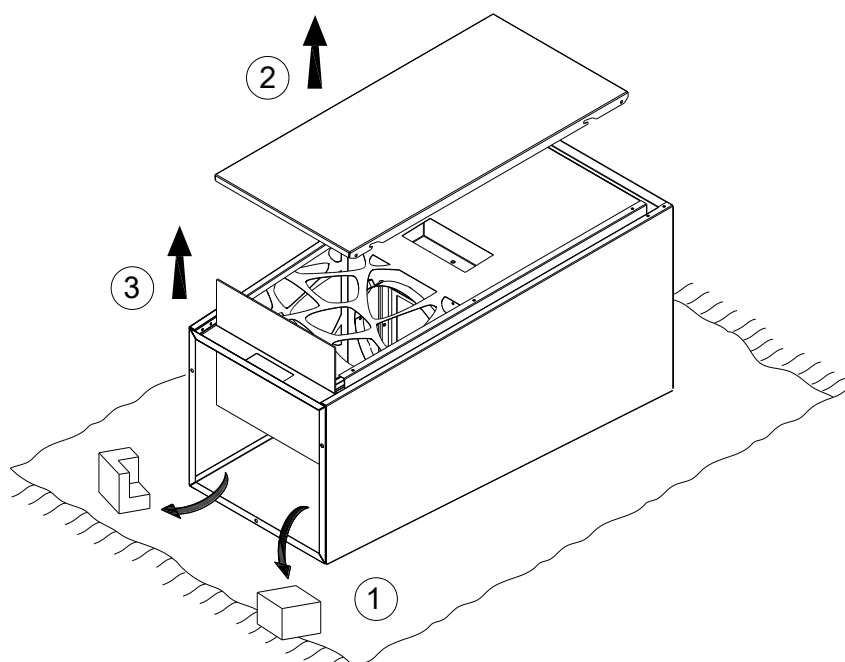
Fig. 4 – Unboxing the fireplace
