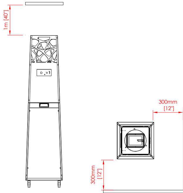
Fig 2 – Minimum distances
